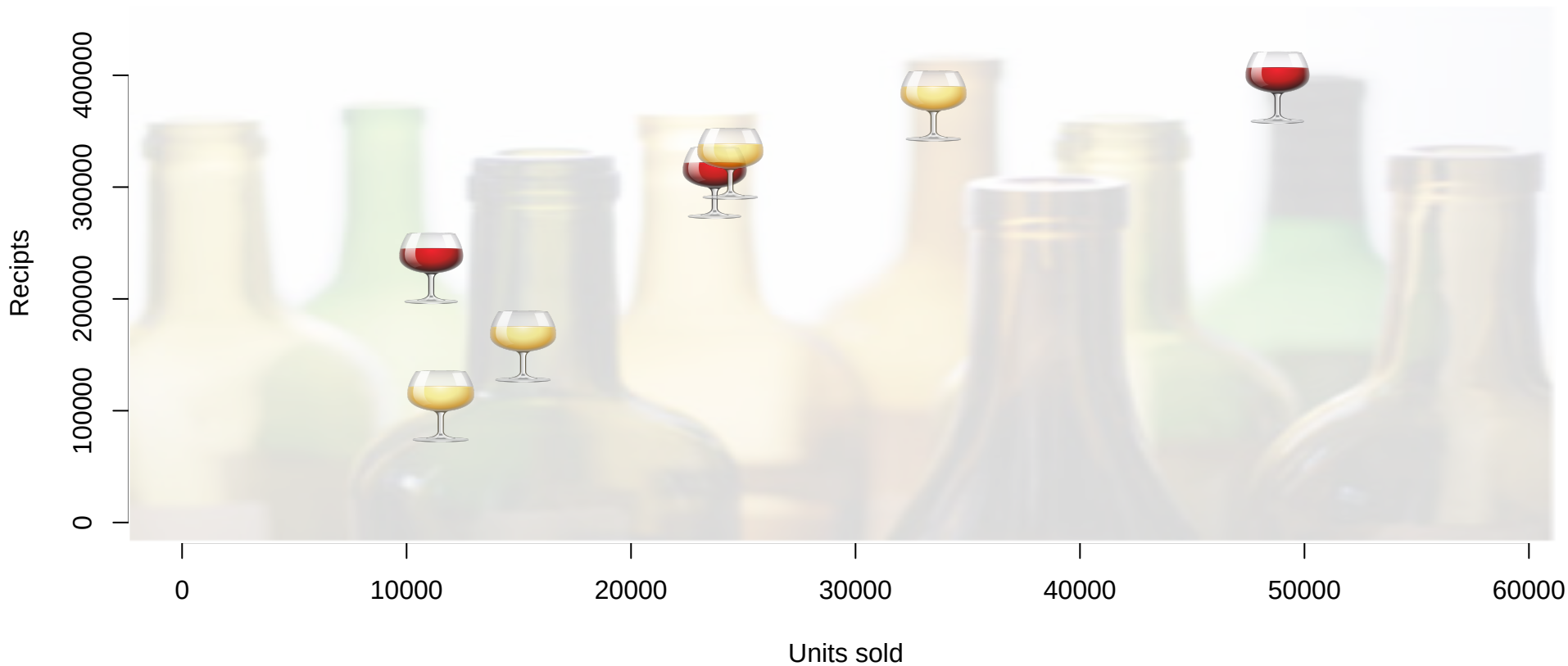
IST421 Simulated Wine Sales Dataset
