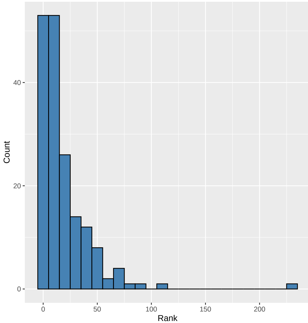
Adjusted Offensive Efficiency Rank
