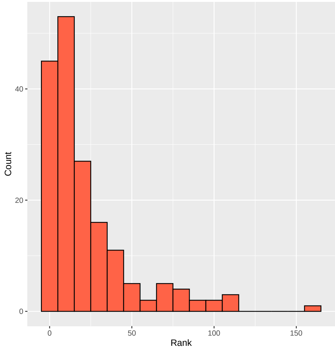
Adjusted Defensive Efficiency Rank
