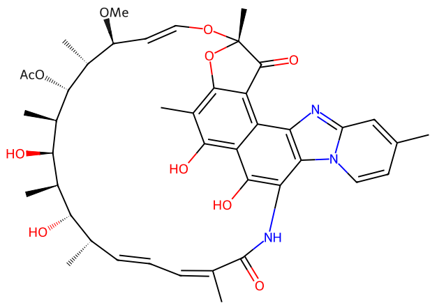
261 rifaximin
