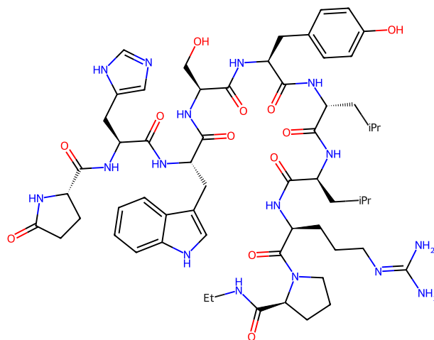
300 leuprolide
