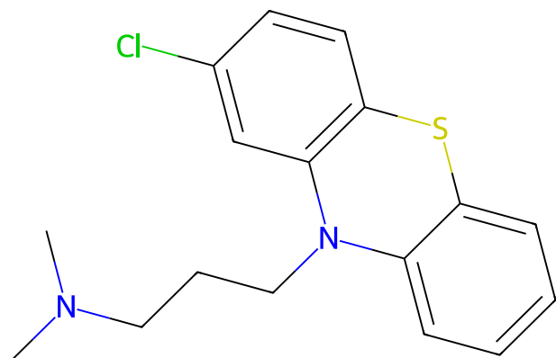
59 chlorpromazine
