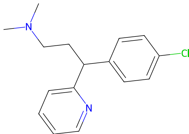
57 chlorpheniramine
