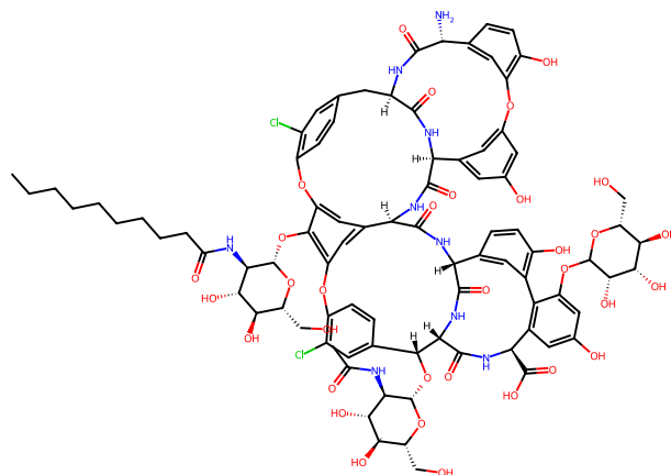
325 teicoplanin
