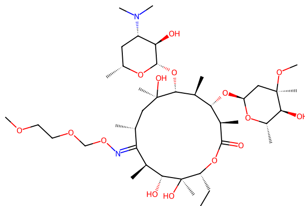
321 roxithromycin
