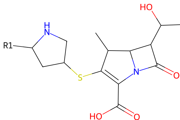
463 scaffold of ertapenem
