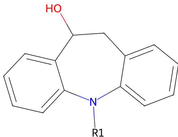
464 scaffold of eslicarbazepine
