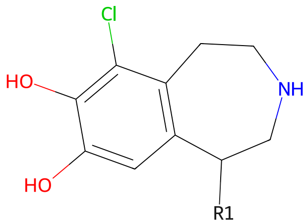
468 scaffold of fenoldopam
