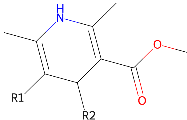
467 scaffold of felodipine
