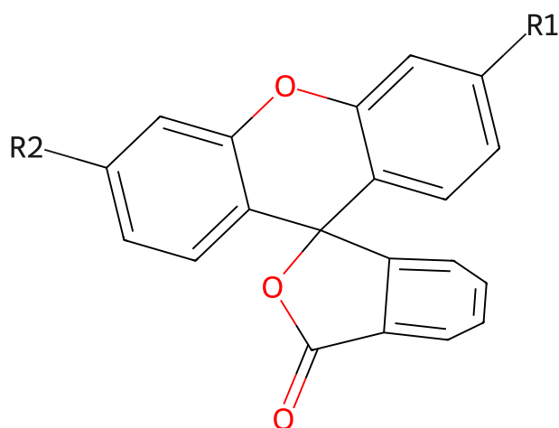
473 scaffold of fluorescein
