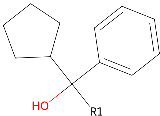
484 scaffold of glycopyrronium
