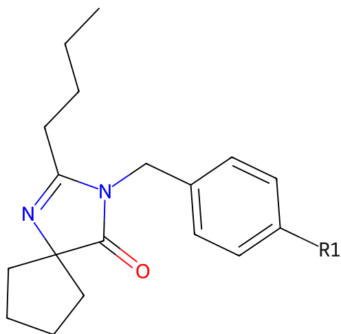
496 scaffold of irbesartan
