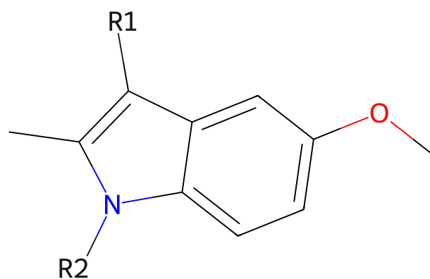
495 scaffold of indomethacin
