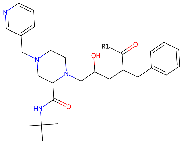
494 scaffold of indinavir
