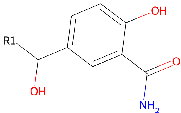
502 scaffold of labetalol
