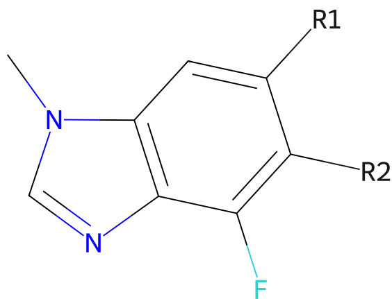
501 scaffold of koselugo
