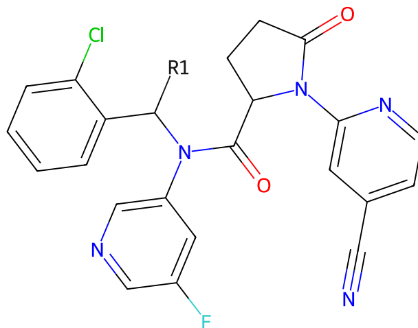
499 scaffold of ivosidenib
