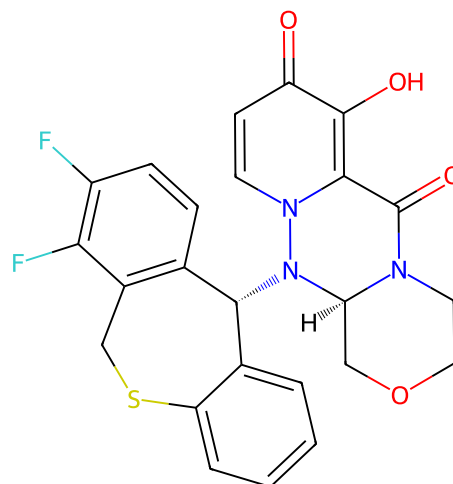
122 baloxavir
