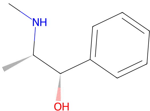
117 pseudoephedrine
