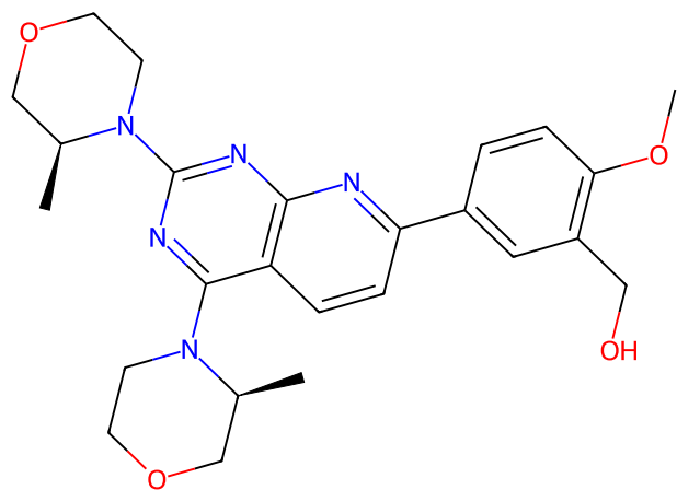
119 azd8055
