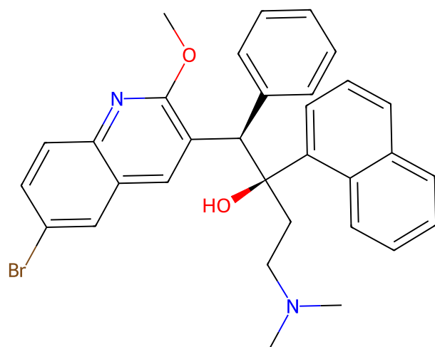
125 bedaquiline
