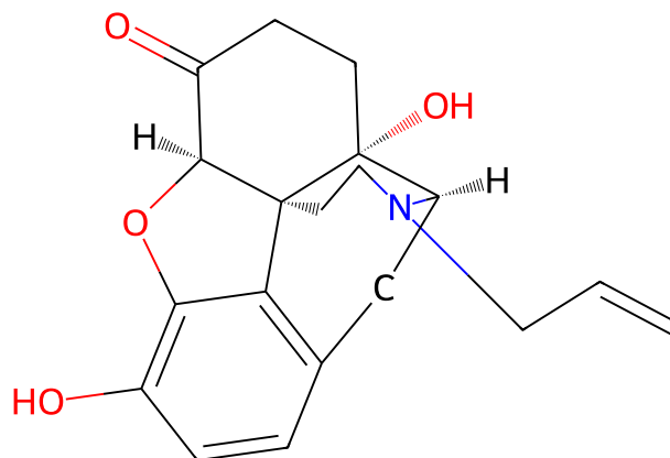
134 naloxone
