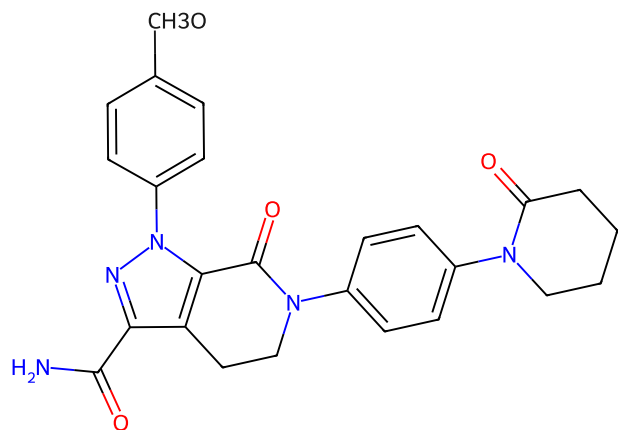
924 apixaban
