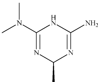
R-Imeglimin -L- amino acid salt
