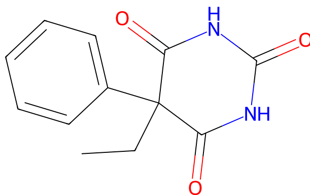
92 phenobarbital
