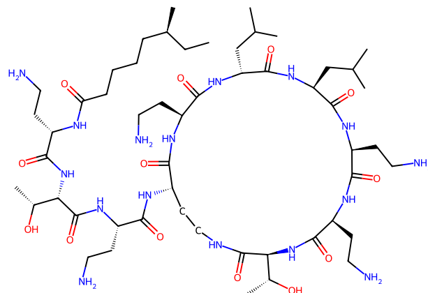
98 colistin A
