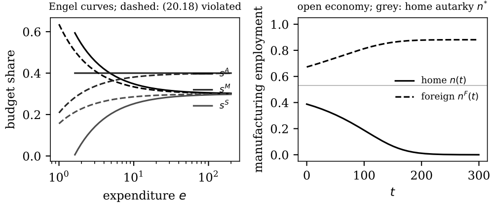
FIGURE 16. Left: Engel curves from the Stone–Geary aggregator (20.2); solid curves impose (20.18), which makes s^M exactly constant, dashed curves set \gamma^S = 0 (Exercise 20.1). Right: manufacturing employment in the open-economy Matsuyama model, with the home economy's autarky share marked in grey (Exercise 20.20).
