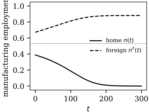
open economy; grey: home autarky n^*
