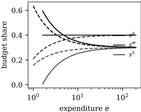
Engel curves; dashed: (20.18) violated
