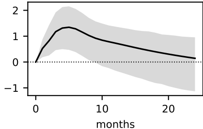
Output to oil-specific demand shock
