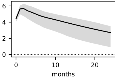
Output to aggregate demand shock
