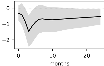
Output to oil supply shock
