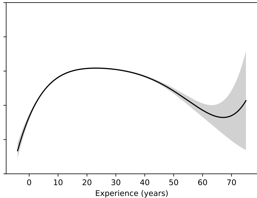
(b) CV-selected order 5
