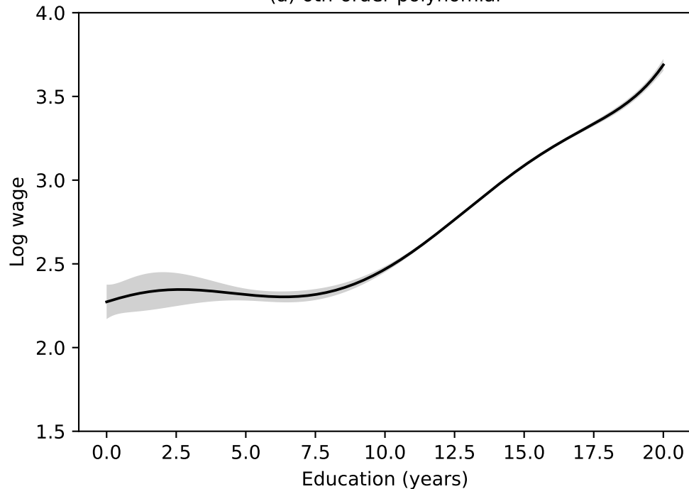
(a) 6th-order polynomial
