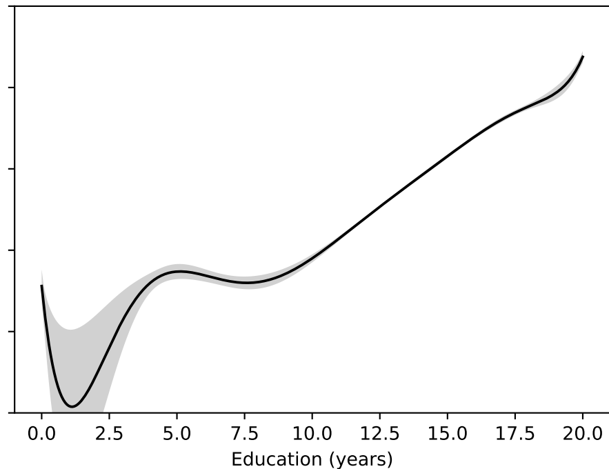
(b) CV-selected order 8
