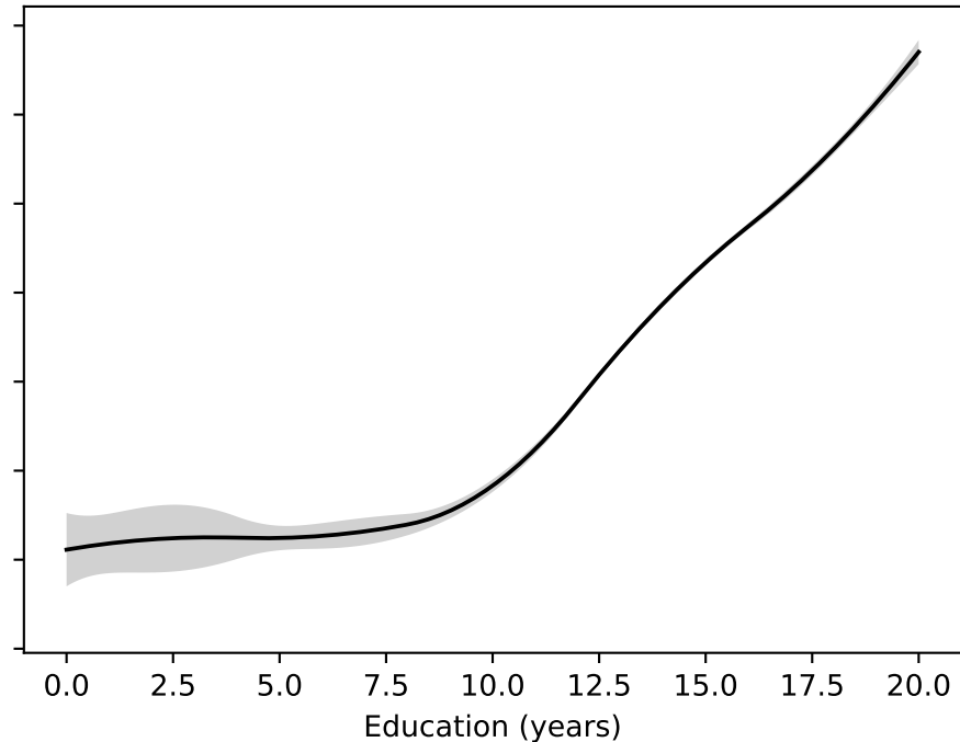
(b) CV-selected spline (knots 4, 8, 12, 16), 95% bands
