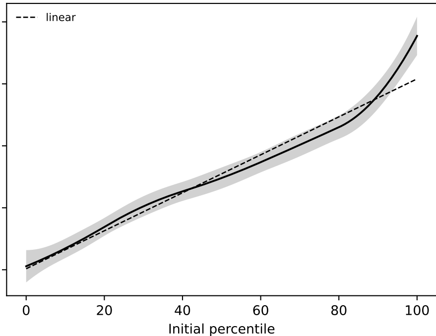
(b) Selected spline (knots 20, 40, 60, 80), clustered 95% bands
