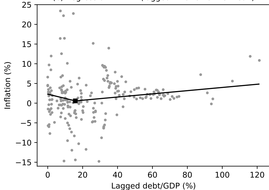
(b) Regression kink fit (lagged inflation at its mean)
