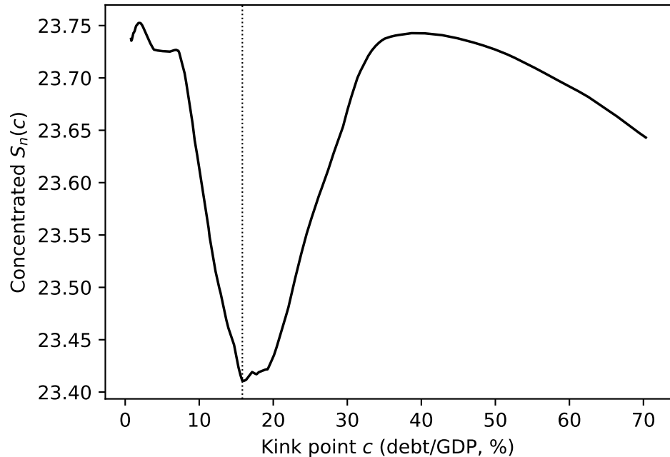
(a) Concentrated least squares criterion
