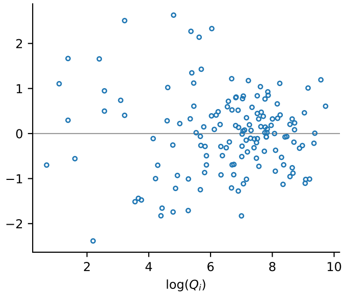
Model 4, weighted residuals
