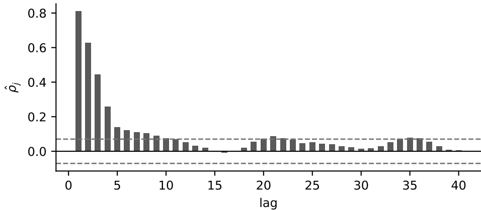
Correlogram of s30 - f , POUND/$
