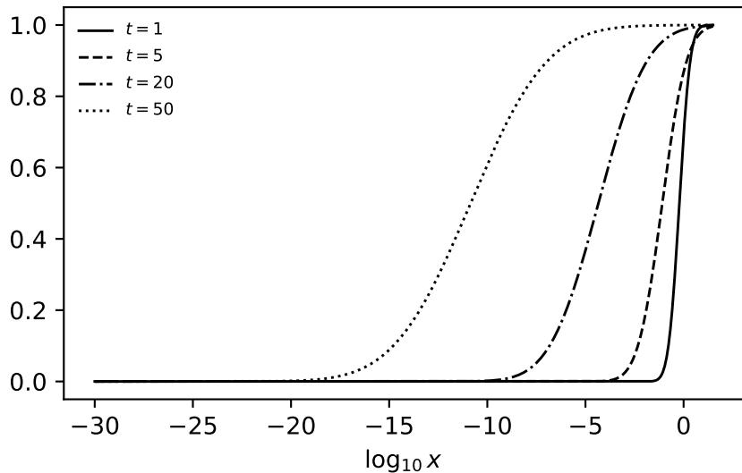
\Pr(\xi_t \leq x) against \log_{10} x
