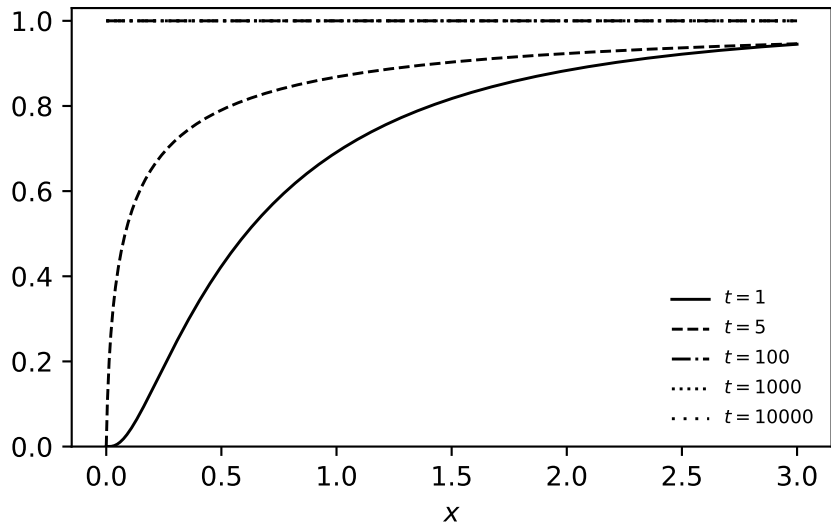
\Pr(\xi_t \leq x)
