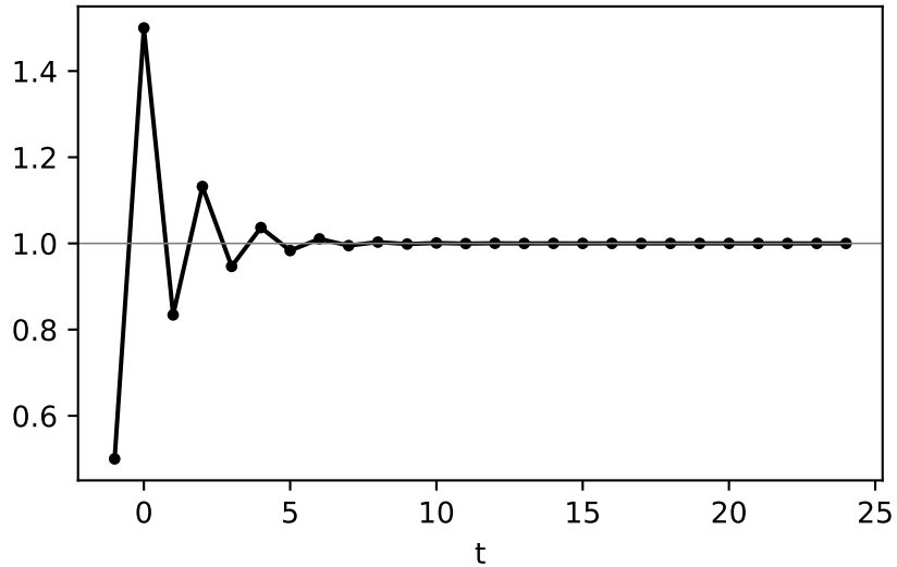
new capital k_t/k^*
