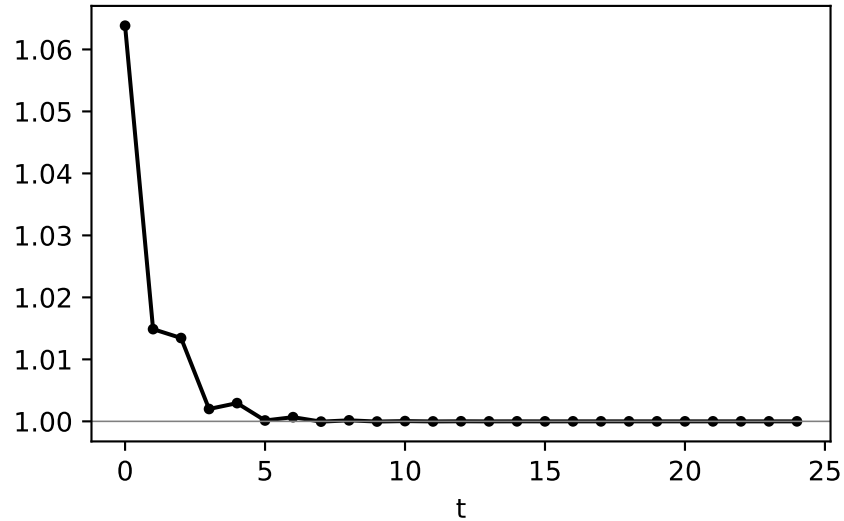
consumption c_t/c^*
