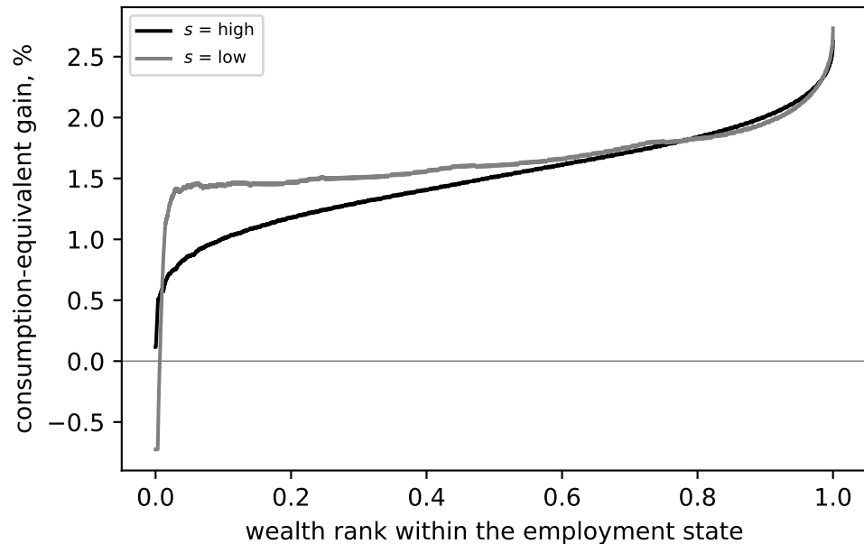
18.6(g): gain from moving to the Bewley equilibrium
