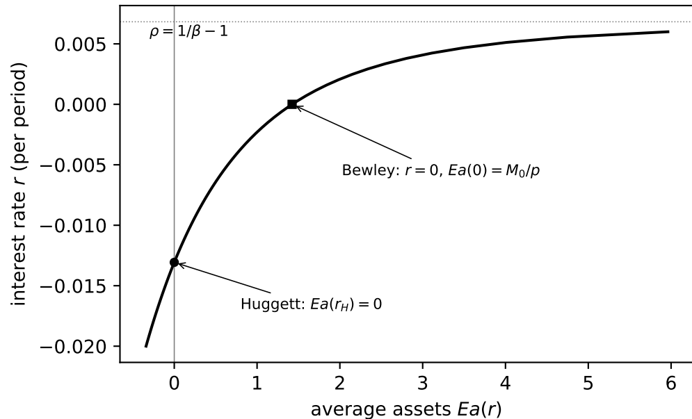
18.6(c): Ea(r) , Huggett parameters, \phi = 2
