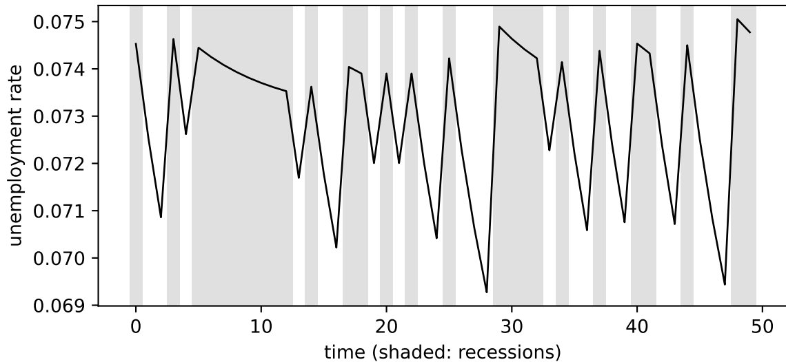
29.2: simulated unemployment with booms and recessions
