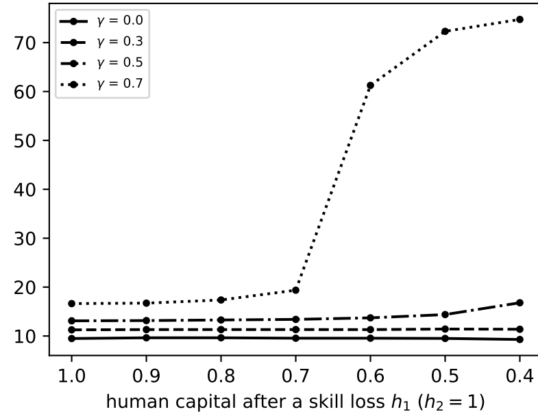
29.6: turbulence and benefits
