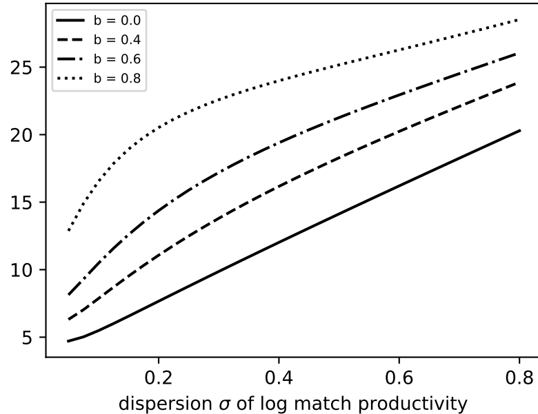
29.5: dispersion of match values
