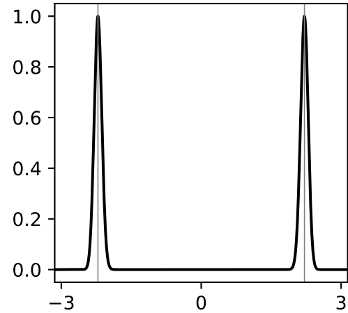
m=120, n=30
