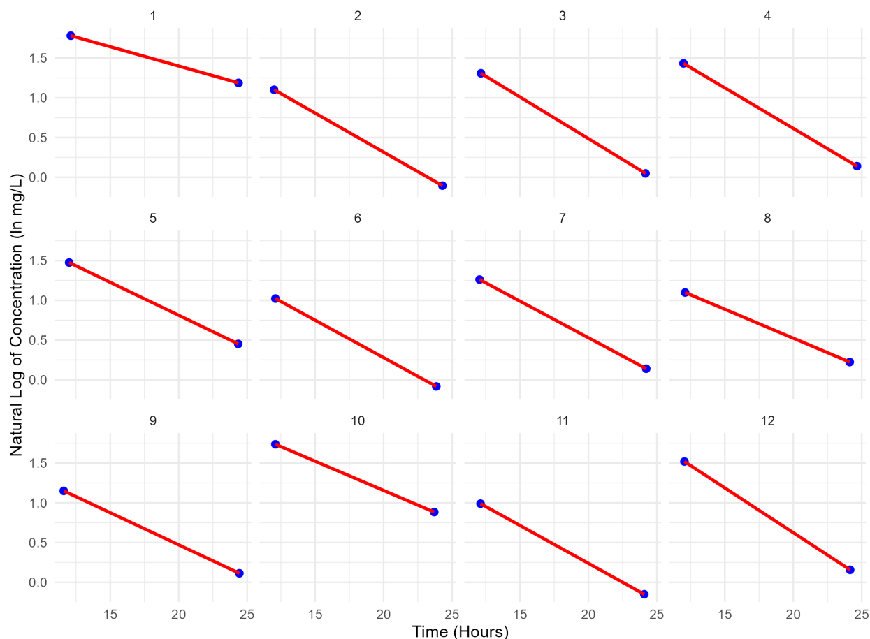
Figure 2: Individual theophylline log-concentration time curves for subjects 1-12. The blue dots represent the individual blood concentration measurements taken for each person during the elimination phase. The red solid lines represent the terminal elimination phase used for the calculation of the elimination rate constant( K_{el} ).
