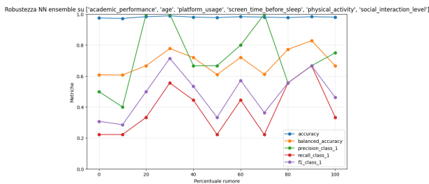
(a) Neural Network, feature peggiori
