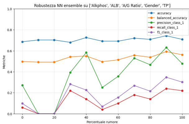
(a) Neural Network, feature peggiori
