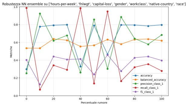
(a) Neural Network, feature peggiori
