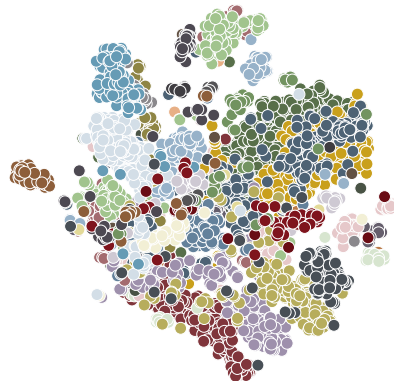
ResNet18 ImageNet
