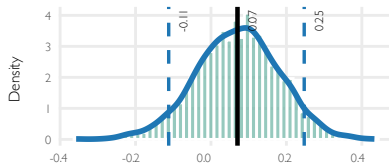
deviance
