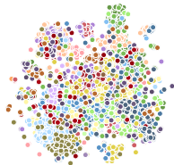
HawkEars
