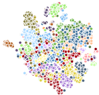
ResNet18-ImageNet
