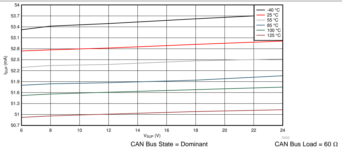
Figure 108. I_{SUP} Across V_{SUP} and Temperature
