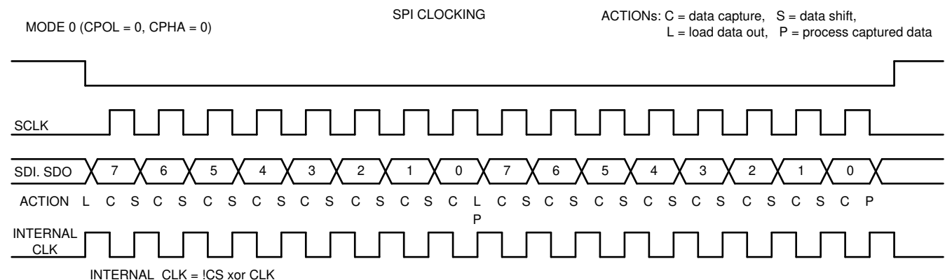
Figure 33. SPI Clocking
