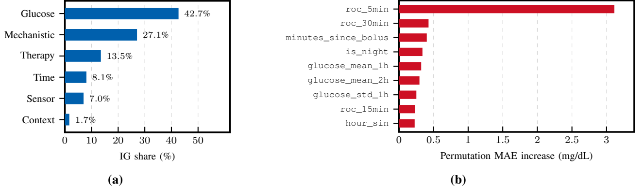
Fig. 7. Feature attribution at 30 min using integrated gradients (a) and permutation importance (b). Glucose-derived features dominate IG attribution (42.7%), while roc_5 is the strongest permuted feature ( \sim 3.1 mg/dL MAE increase). Both methods identify glucose dynamics as the leading predictors.
