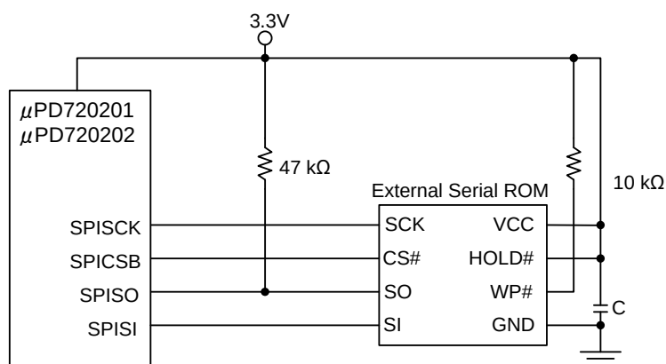
Figure 5-7. External Serial ROM Connection
