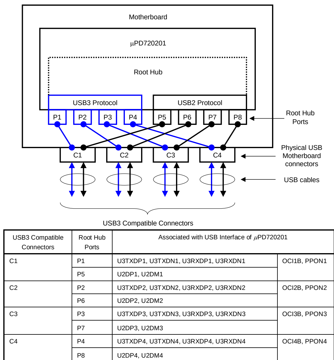
Figure 5-1. Root Hub Port to USB Connector Mapping of μPD720201
