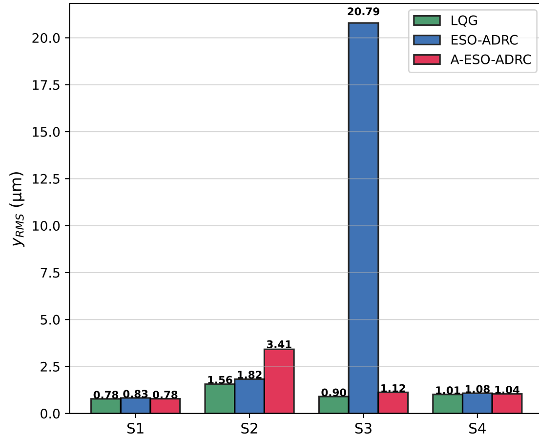
Vibration RMS
