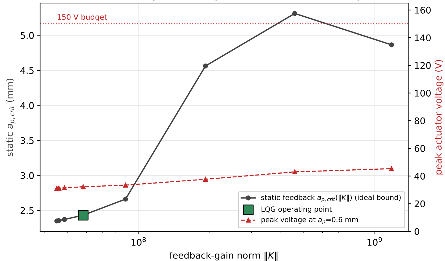
Feedback authority vs stability (static bound) and voltage cost
