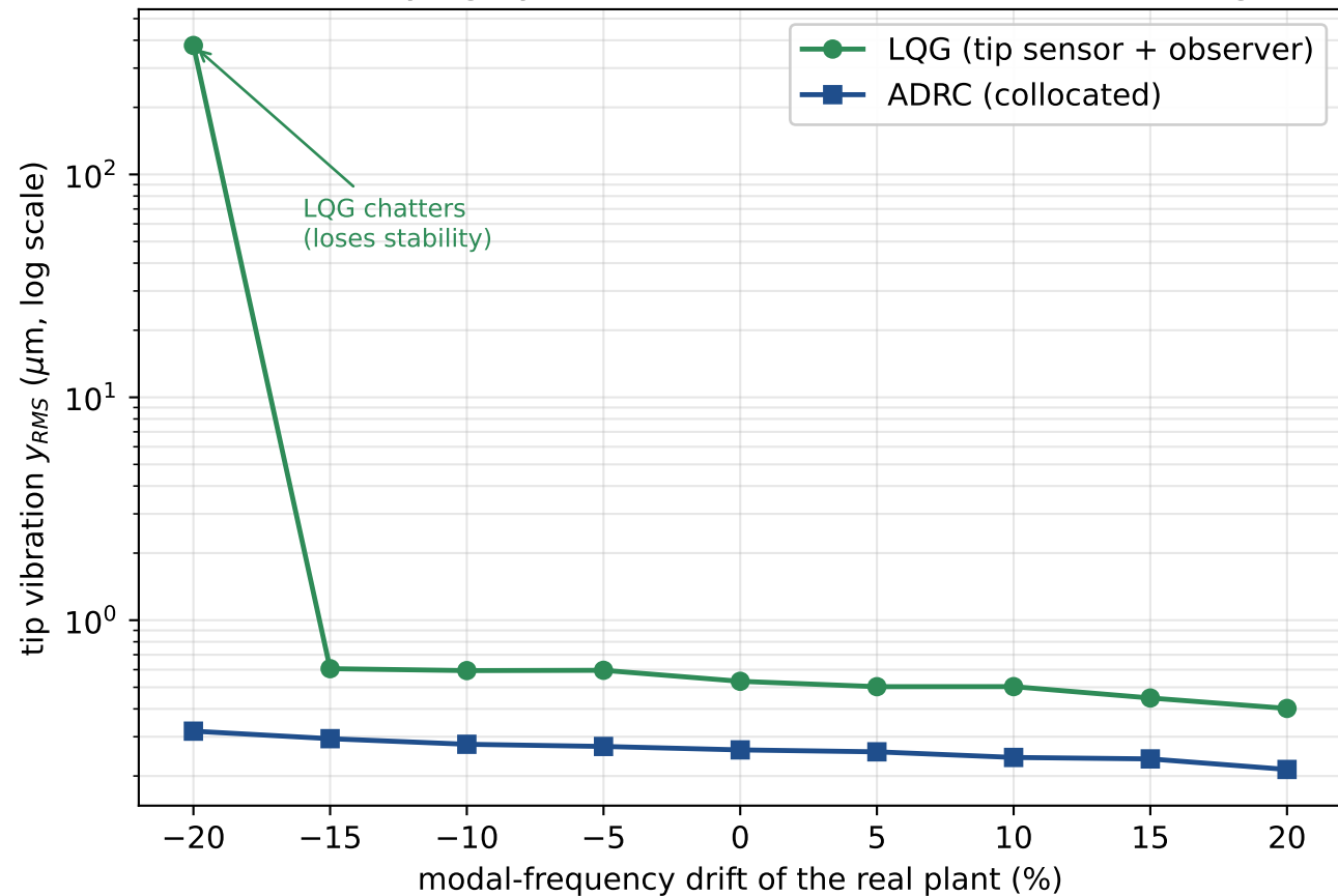
Robustness to varying dynamics: model-based LQG vs model-light ADRC
