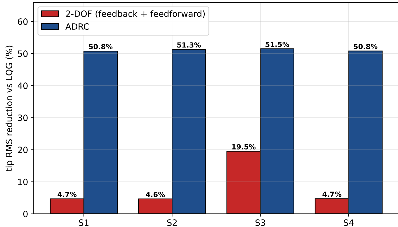
Vibration reduction relative to the LQG baseline
