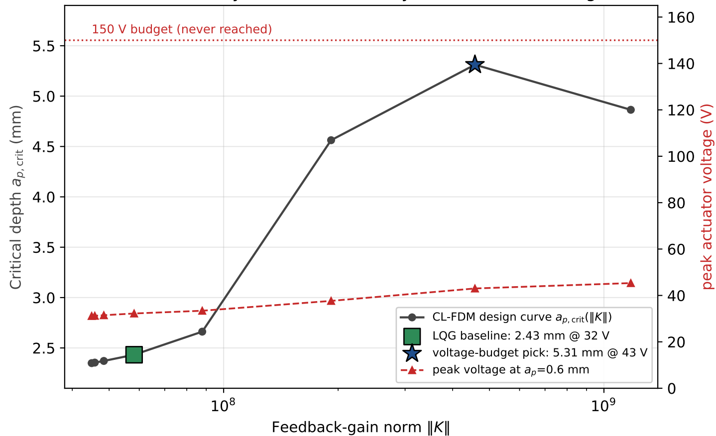
Feedback authority vs chatter stability (CL-FDM) and voltage cost
