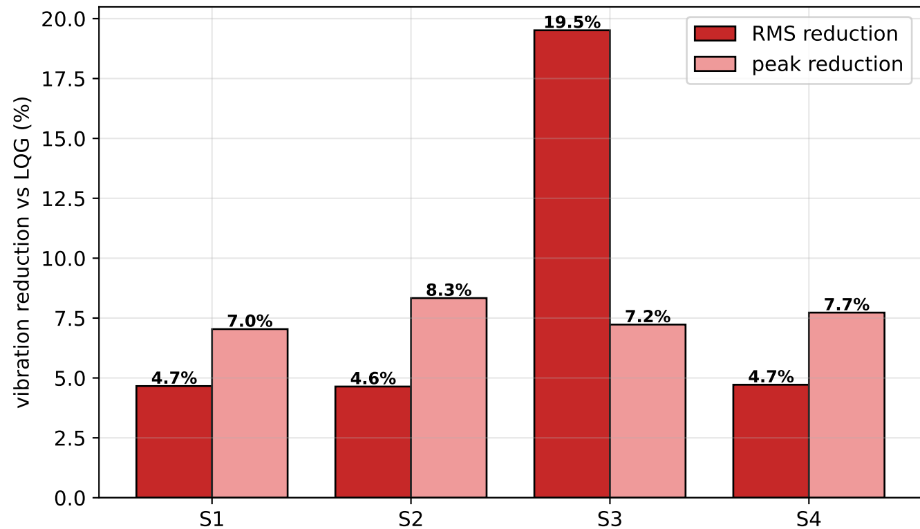
Phase-aware feedforward: measured reduction (2-DOF vs LQG)
