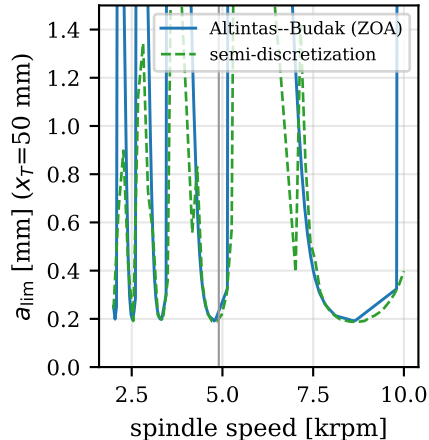
(c) open-loop lobes (classical model)
