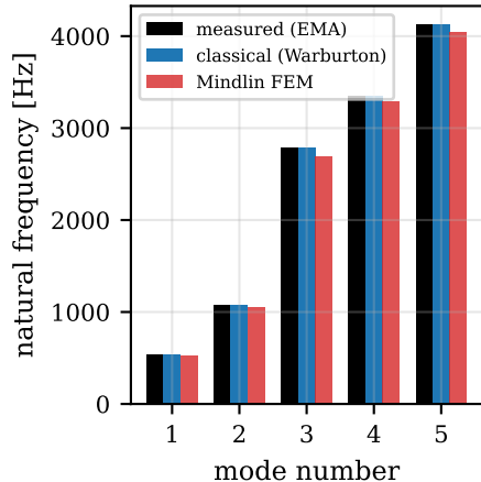
(a) modal frequencies
