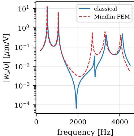
(b) actuator FRF (at sensor)
