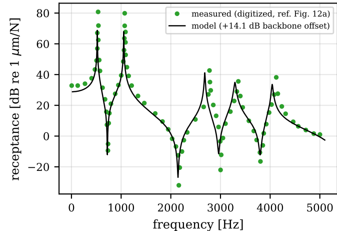
(a) impact receptance, structure match
