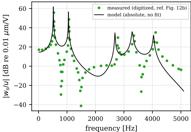
(b) piezo transfer function, absolute
