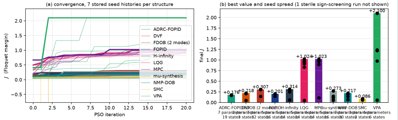
PSO optimisation - 2646-5586 evaluations, swarm scaled with the parameter count, identical seeds, identical objective Protocol B - design and evaluation on the full 5-mode model
