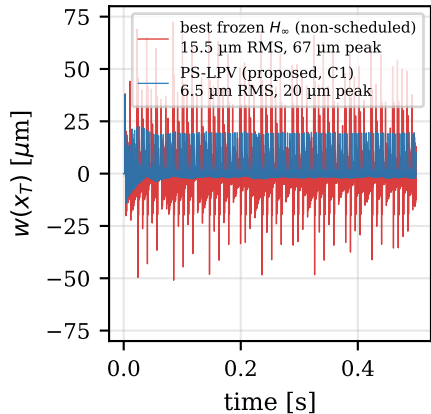
(a) milling-point displacement (open loop & delayed PD diverge here)
