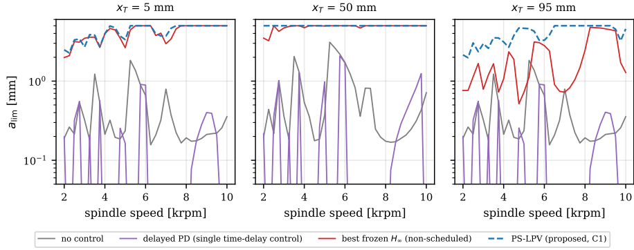
Figure 7: Closed-loop stability lobe diagrams at three tool positions on the 12-mode evaluation model: open loop, delayed PD (tuned at the reference speed; note its destabilized bands at other speeds), best-frozen H_\infty , and the scheduled PS-LPV controller. PS-LPV-DR is not drawn: its certified delayed gain is zero (Section 5.5), so it reproduces the PS-LPV lobes exactly.
